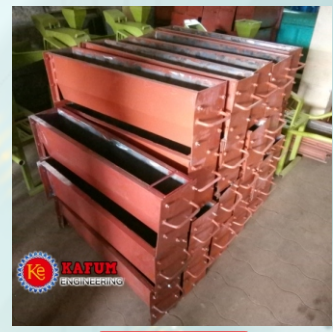
Road kerb moulds
